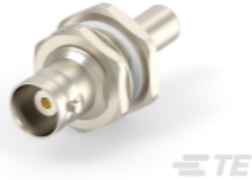
TE Part # 6-1337433-0 BNC RM BHj Hex 50Ohm Nickel Pltd RG58C/U
